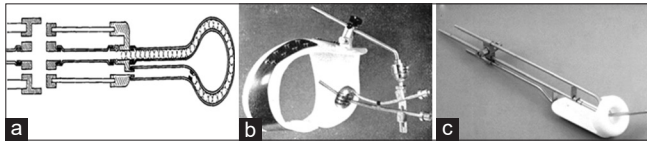
Supplementary Figure 7: Ring applicator. (a and b) Schematic diagram of early ring applicator for cervitron II and remote afterloading machine. [36,38] (c) Applicator with rectal retractor for nucletron machine [39]
